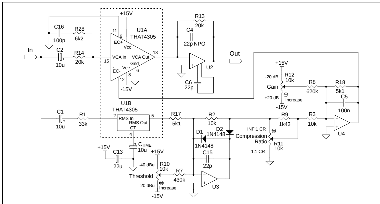
Figure 16. 4305-based feedforward compressor
